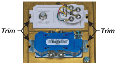
IMPORTANT: Trim receptacle mount tabs
