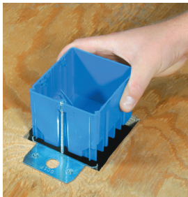
Install clip over subfloor.
