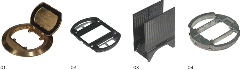
01 Duplex cover 02 Faceplate 03 Dual-voltage divider 04 Mounting ring
